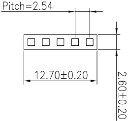
HOUSING
