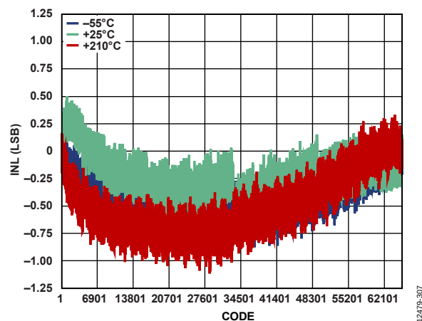
Figure 9. Integral Nonlinearity (INL) vs. Code and Temperature, V_{REF} = 5.0\text{ V} , FLATPACK
