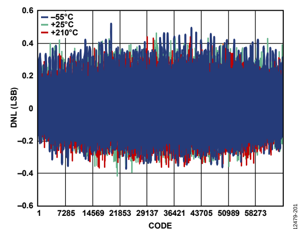
Figure 11. Differential Nonlinearity (DNL) vs. Code and Temperature, V_{REF} = 5.0\text{ V} , FLATPACK
