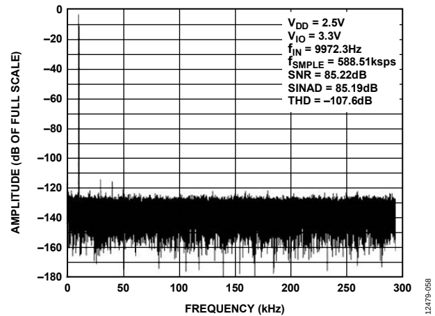
Figure 21. 10 kHz FFT, V_{REF} = 2.5\text{ V}
