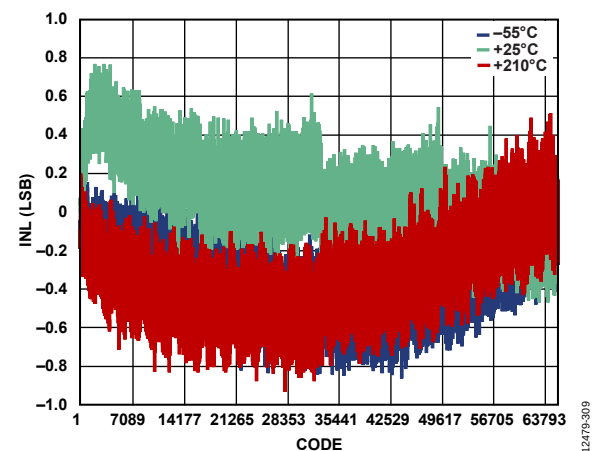
Figure 10. Integral Nonlinearity (INL) vs. Code and Temperature, V_{REF} = 2.5\text{ V} , FLATPACK
