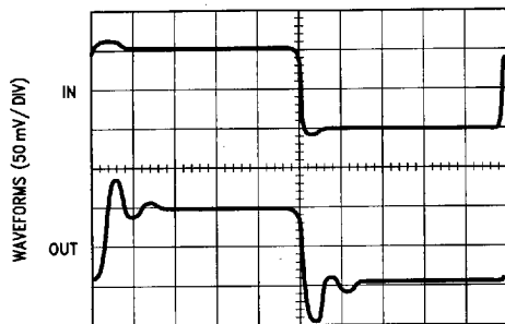
Small Signal, Non-Inverting T_A = 25^\circ\text{C} , A_V = 1 , R_L = 600\Omega , V_S = \pm 15\text{V}
