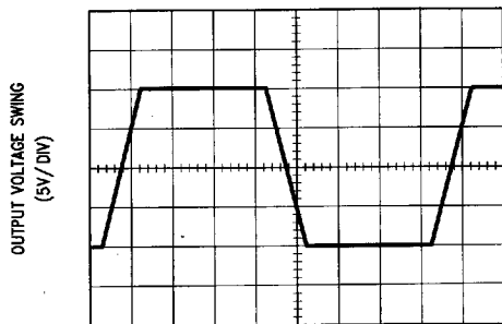
Large Signal Non-Inverting T_A = 25^\circ\text{C} , R_L = 600\Omega , V_S = \pm 15\text{V}
