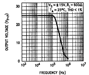
Power Bandwidth
