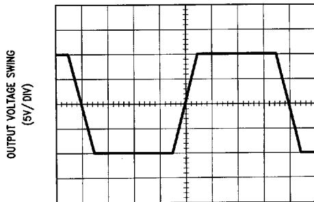
Large Signal Inverting T_A = 25^\circ\text{C} , R_L = 600\Omega , V_S = \pm 15\text{V}
