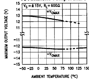
Maximum Output Voltage vs Ambient Temperature
