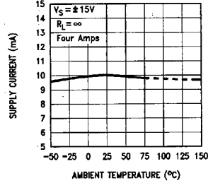
Supply Current vs Ambient Temperature
