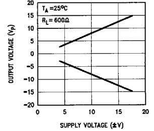
Maximum Output Voltage vs Supply Voltage
