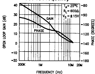
Open Loop Gain & Phase vs Frequency
