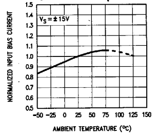
Normalized Input Bias Current vs Ambient Temperature
