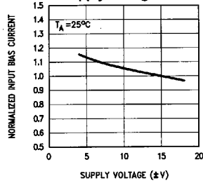
Normalized Input Bias Current vs Supply Voltage
