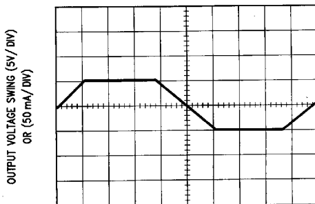
Current Limit T_A = 25^\circ\text{C} , V_S = \pm 15\text{V} , R_L = 100\Omega , A_V = 1
