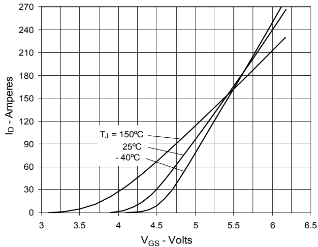
Fig. 7. Input Admittance
