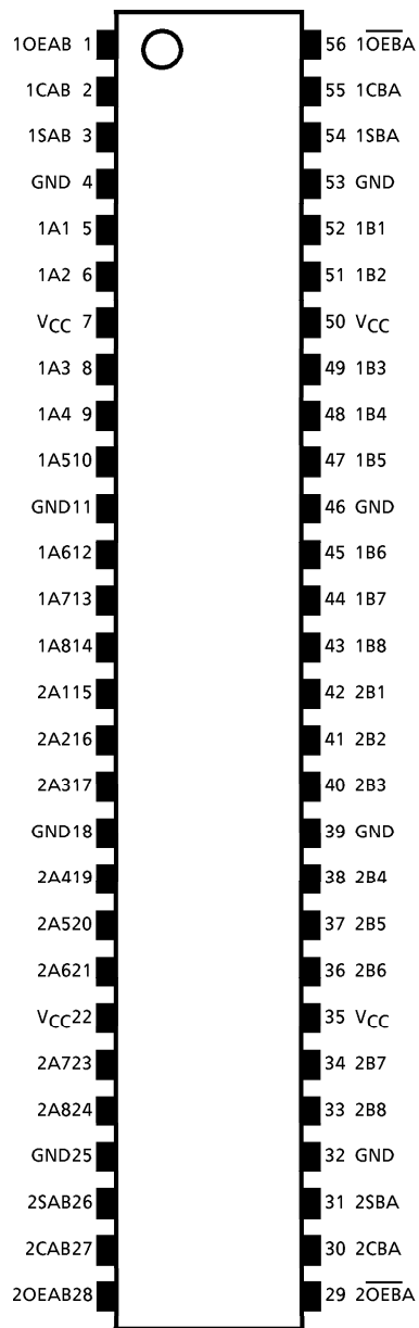
(TOP VIEW)
