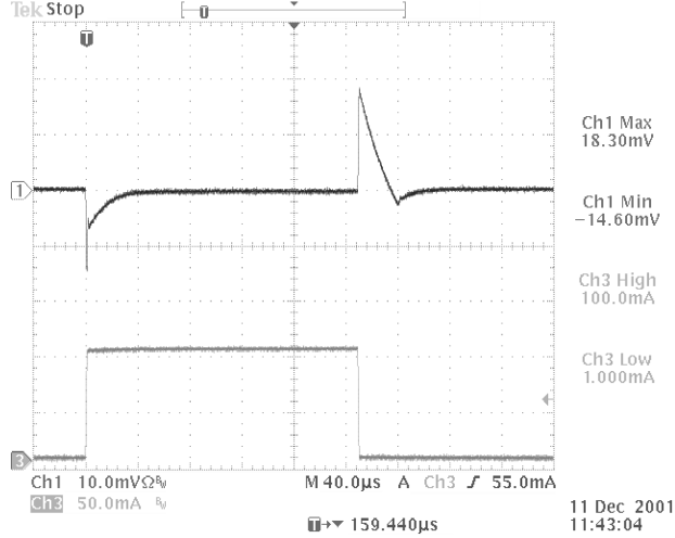
Load regulation of LDO1
