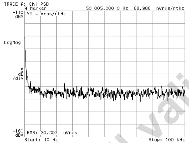
Output noise of LDO1
