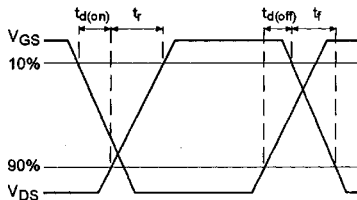
Fig. 17b — Switching Time Waveforms
