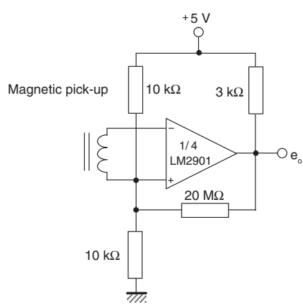
Figure 13. Transducer amplifier
