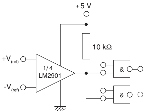
Figure 10. Driving TTL
