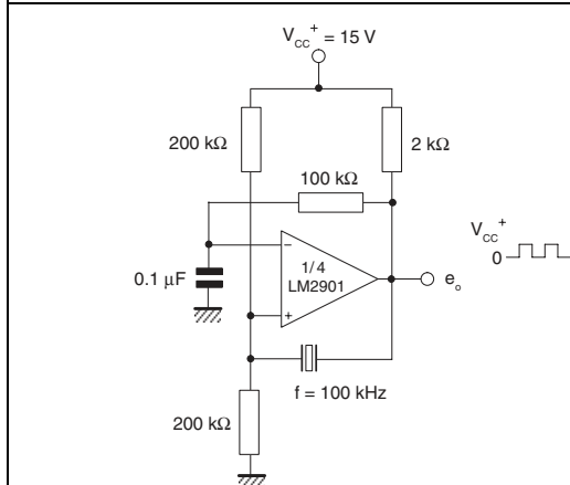
Figure 18. Crystal controlled oscillator
