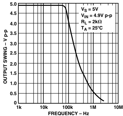
TPC 19. Closed-Loop Output Voltage Swing vs. Frequency
