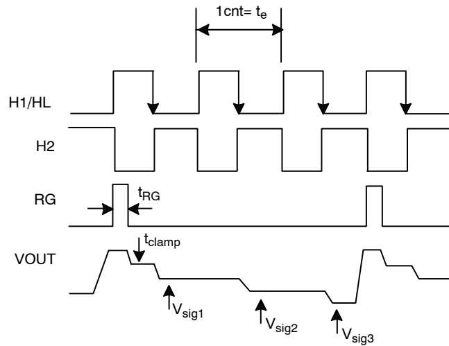
Figure 25. Pixel Timing (3x3 Binning)
