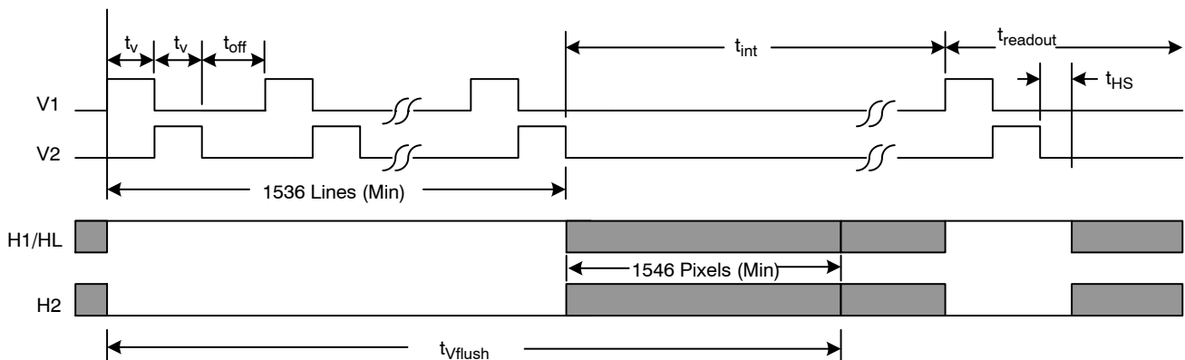
Figure 26. Flush Timing
