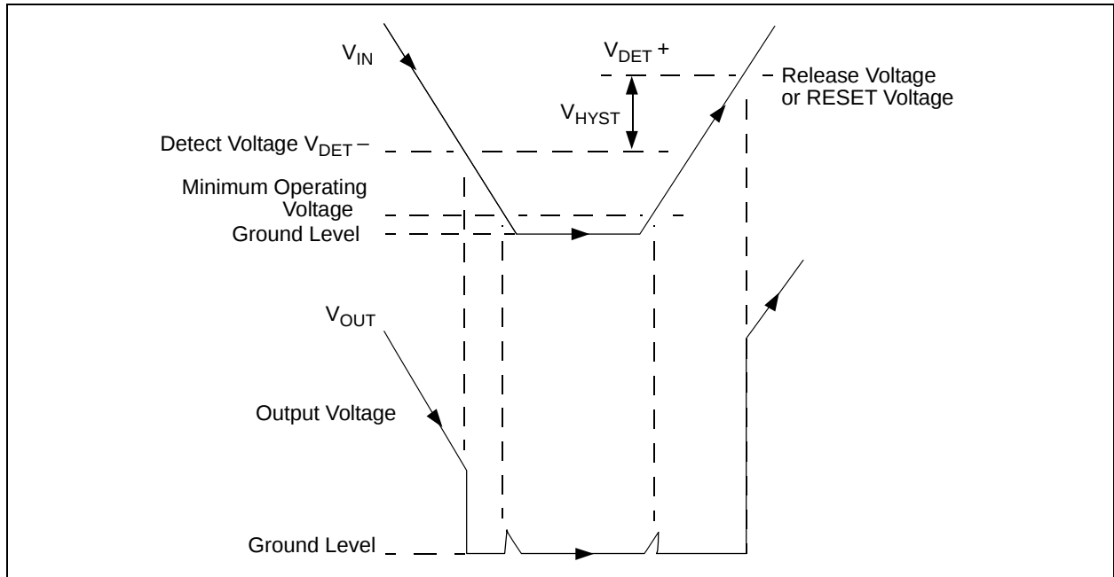
FIGURE 3-1: Timing Diagram.
