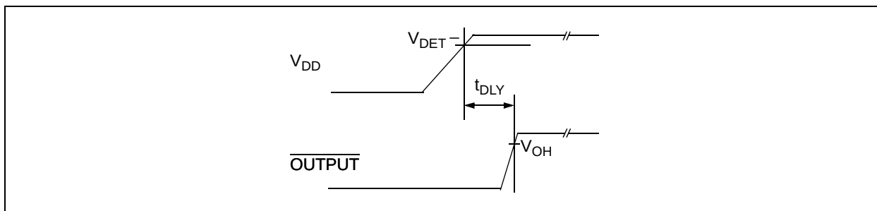
FIGURE 1-1: Timing Diagram.
