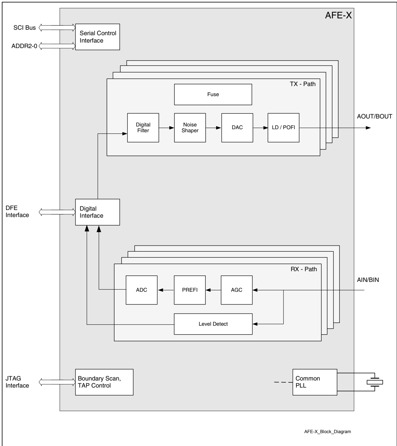
Figure 4 Block Diagram
