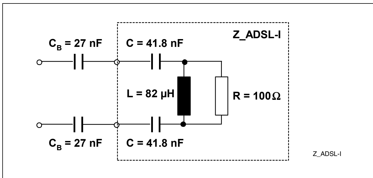
Figure 12 Terminating Impedance of the ADSL Port Z_{\text{ADSL-I}}
