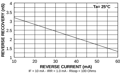
REVERSE RECOVERY TIME vs REVERSE CURRENT
