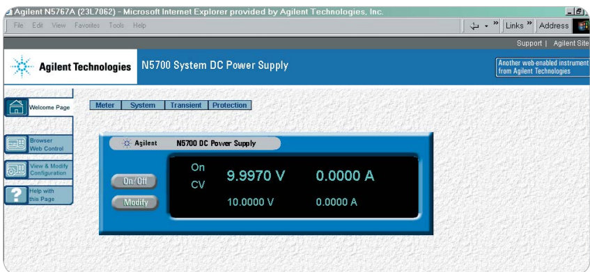
Figure 3. N5700 series web graphical user interface for remote access and control of the power supply.
