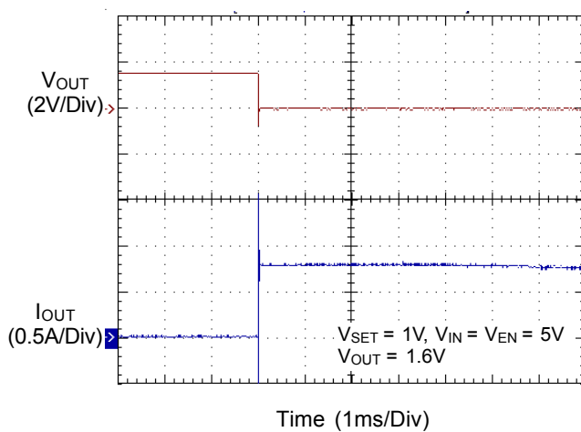
Short-Circuit Protection
