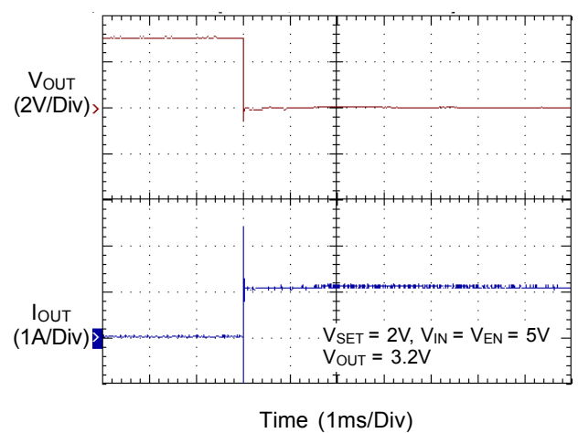
Short-Circuit Protection
