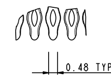
DETAIL T SCALE 5.000
