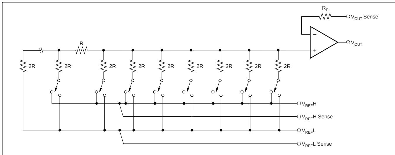
FIGURE 1. DAC7744 Architecture.
