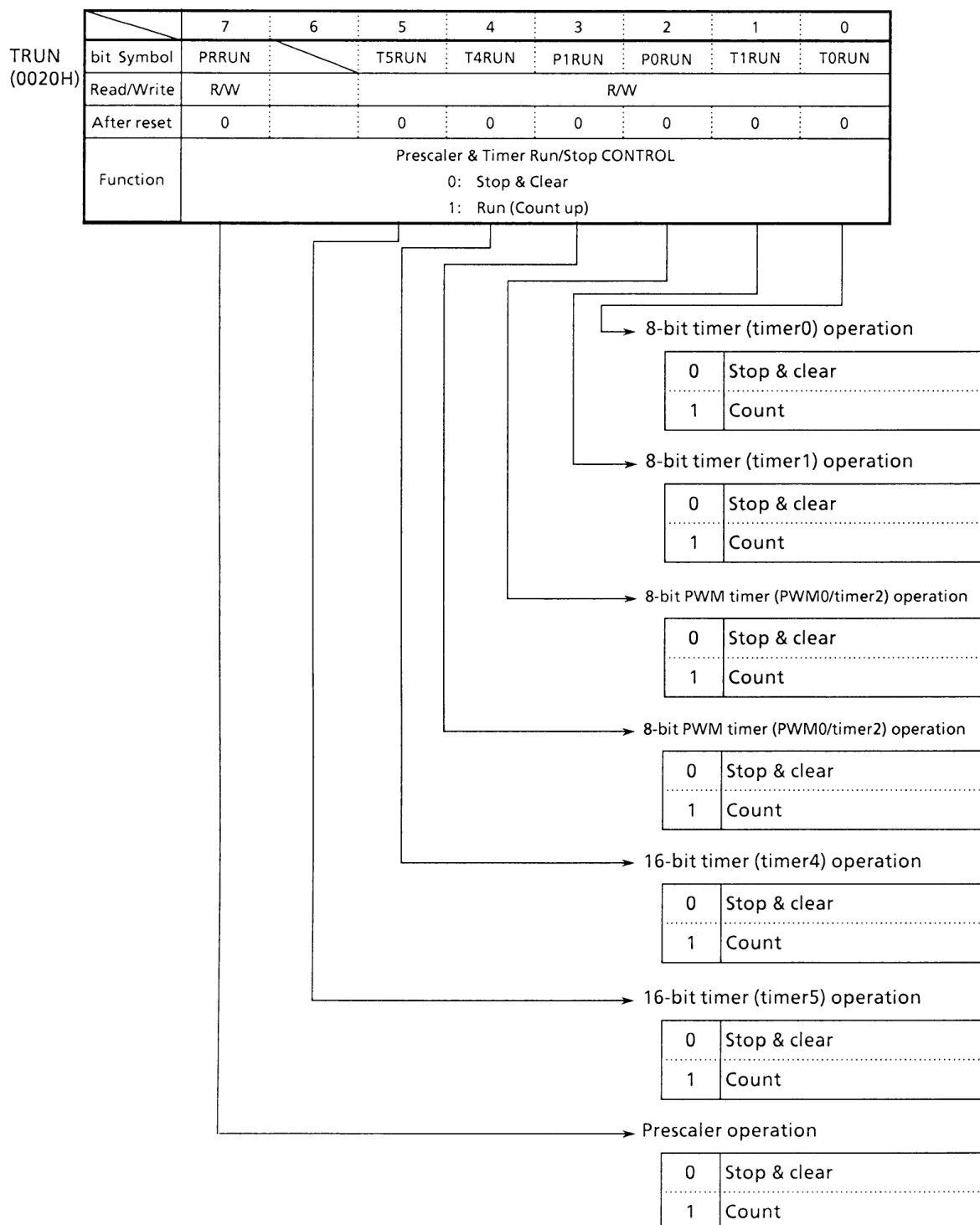
Figure 3.8 (7). Timer Operation Control Register (TRUN)
