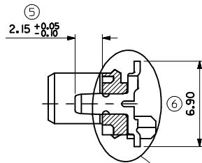
SECTION Y-Y
