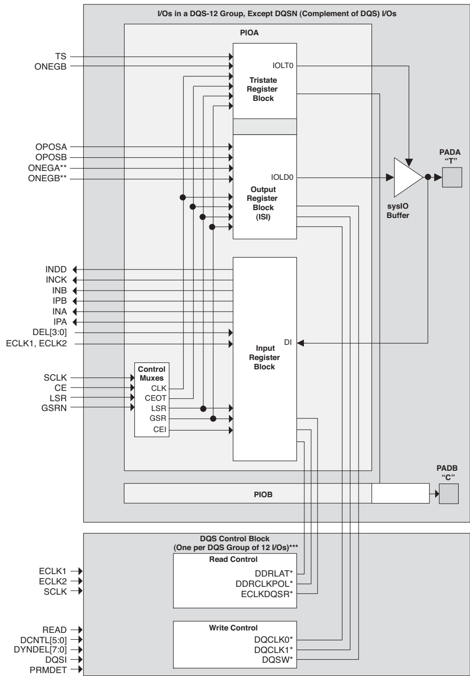
Figure 2-32. PIC Diagram
