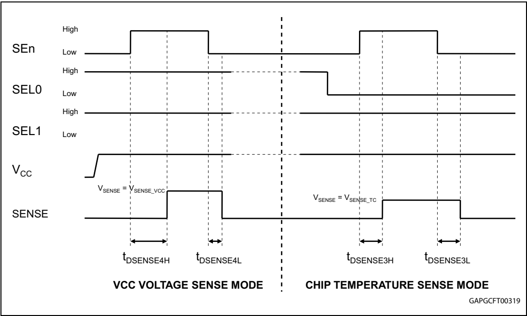
Figure 8. Multisense timings (chip temperature and V_{\text{CC}} sense mode) (VN7040AJ-E only)
