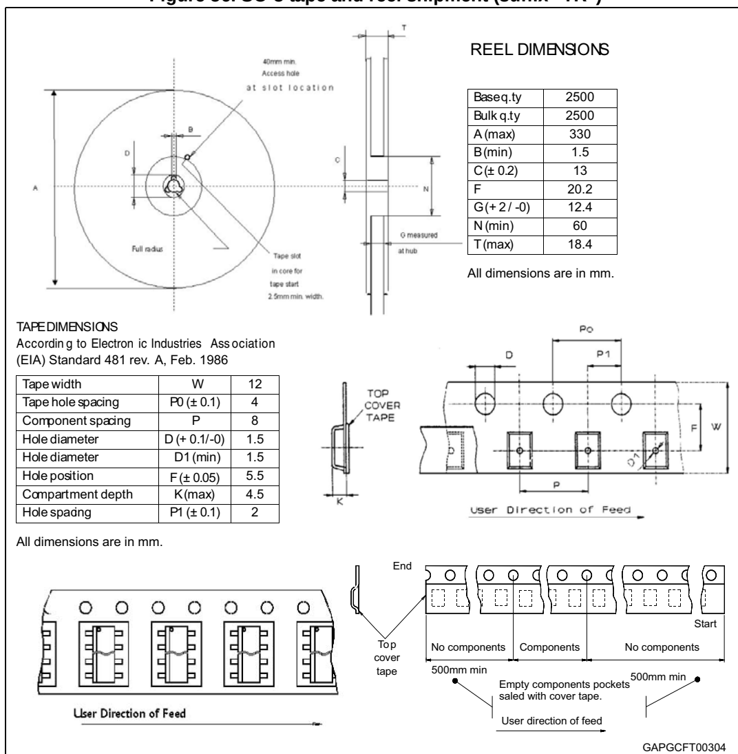
Figure 56. SO-8 tape and reel shipment (suffix "TR")
