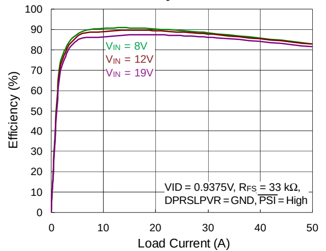
CCM Efficiency vs. Load Current
