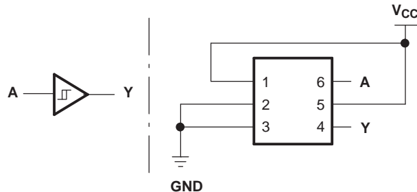
Figure 6. Noninverted Buffer
