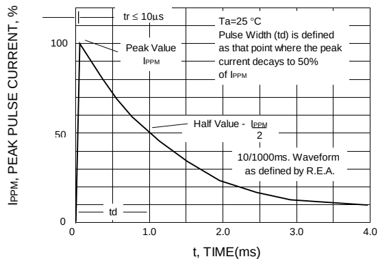
FIG.5 - PULSE WAVEFORM
