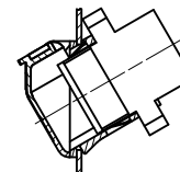
SECTION C-C VERSION 4 (MTP-MTP) SEE NOTE 2
