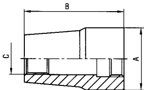
Metal-Backshell with PG thread
