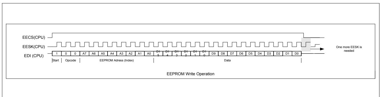
Figure 8 Write EEPROM Registers in the ADM6926 (Index = 2, Data = 16'h2222)
