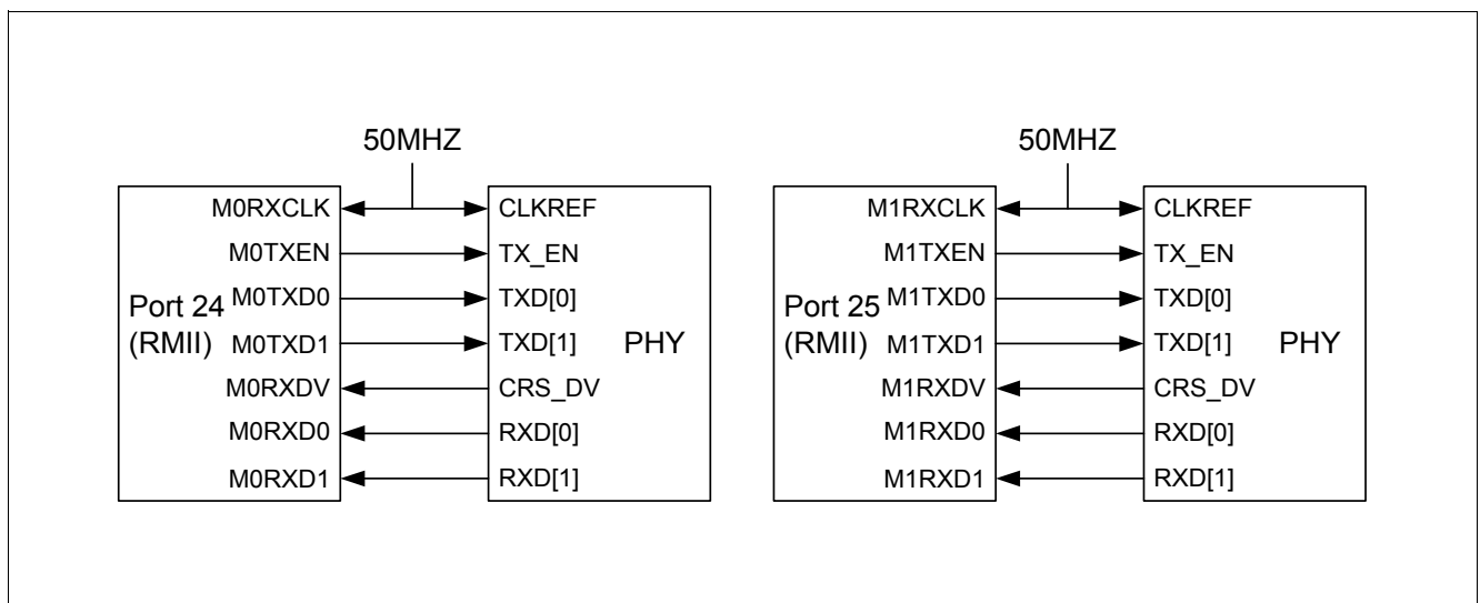
Figure 5 RMII Interface
