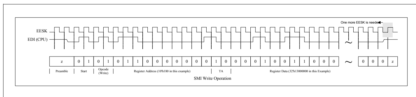
Figure 10 Write Switch Register via SMI Interface
