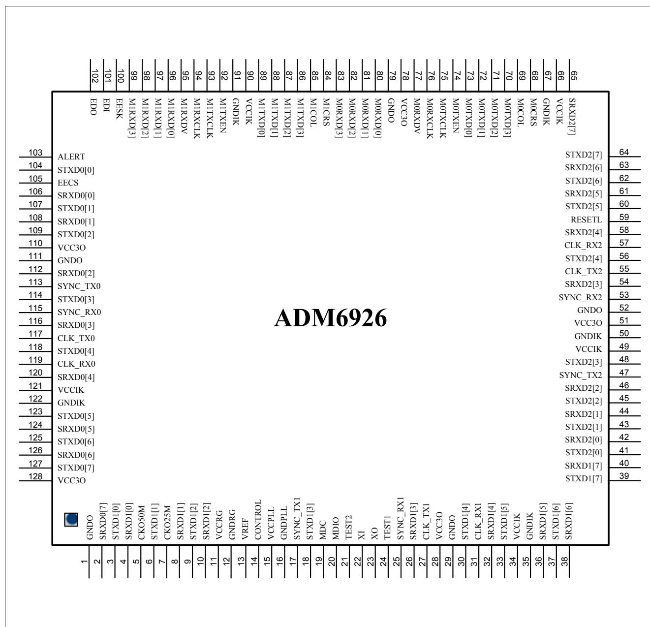
Figure 2 ADM6926 Pin Diagram (SS-SMII Interface)
