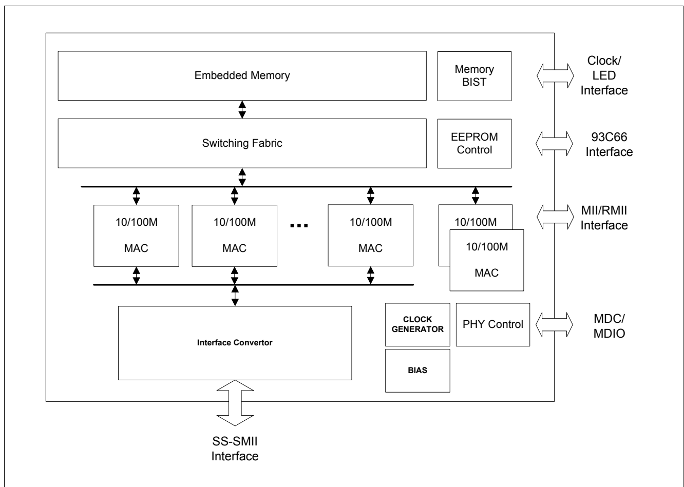
Figure 1 ADM6926 Block Diagram
