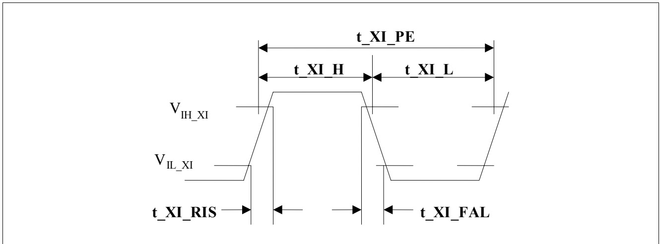
Figure 13 Crystal/Oscillator Timing
