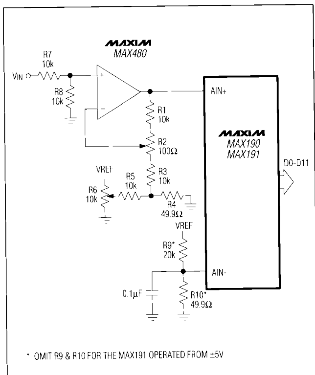
Figure 21b. Offset ( \pm 10\text{mV} ) and Gain ( \pm 1\% ) Trim Circuit
