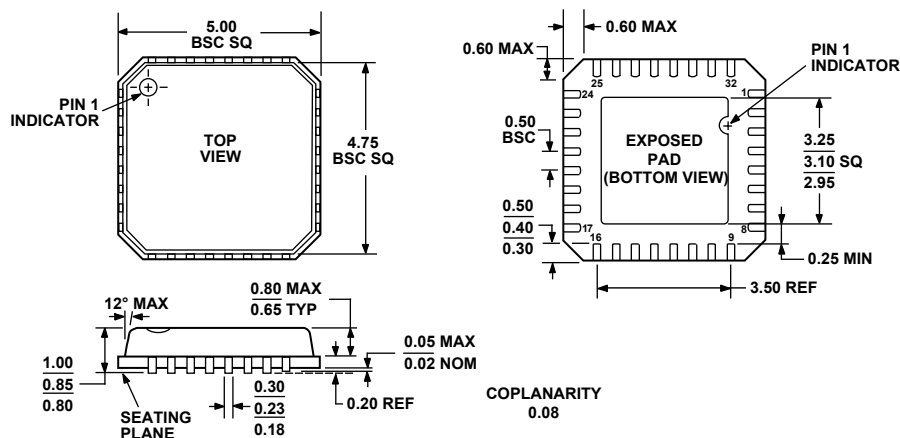
Figure 22. 32-Lead Lead Frame Chip Scale Package [LFCSP_VQ]
