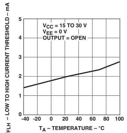
Figure 9. I_{FIH} vs. Temperature.
