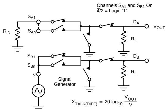
FIGURE 10. Differential Crosstalk
