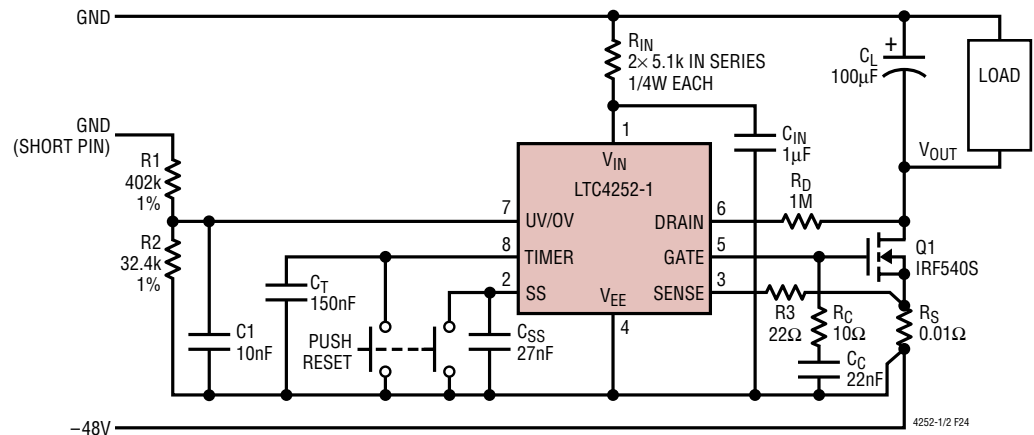
Figure 24. -48V/5A Application
