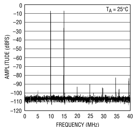
Averaged 8192 Point 2-Tone FFT, 65.2MHz and 70.2MHz Inputs, -7dB, 3.2V Range
