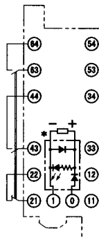
G7SA-4A2B Mounted
