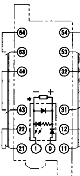
G7SA-3A3B Mounted
