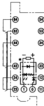
G7SA-5A1B Mounted
