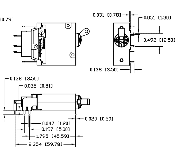
PRINTED CIRCUIT BOARD MOUNTING TERMINAL CODE L
