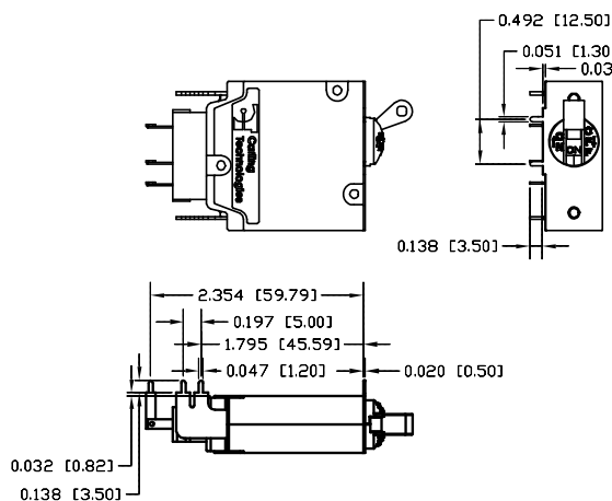
PRINTED CIRCUIT BOARD MOUNTING TERMINAL CODE R
