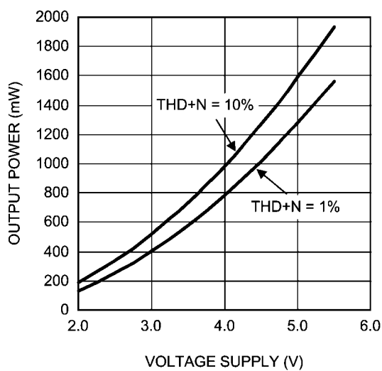
Output Power vs Supply Voltage R_L = 8\Omega
