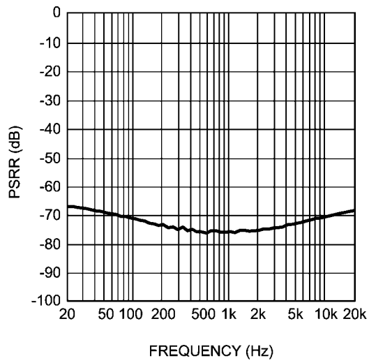
PSRR vs Frequency V_{DD} = 3V , R_L = 8\Omega
