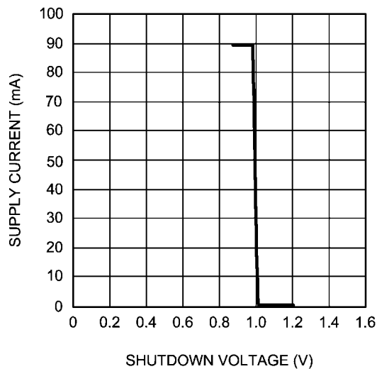
Shutdown Voltage V_{SDIL} V_{DD} = 3V
