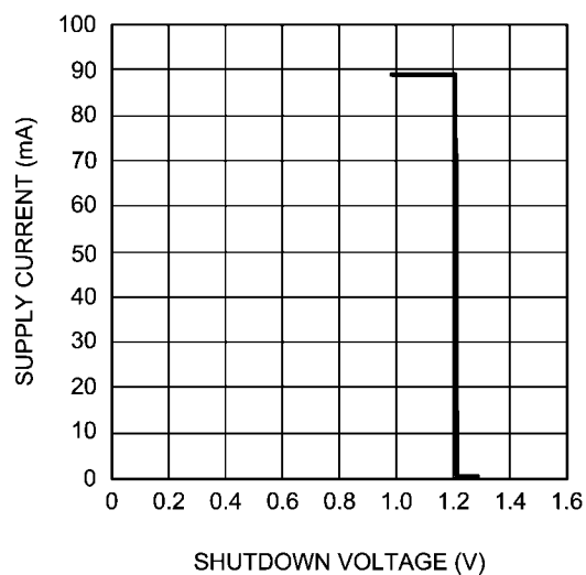
Shutdown Voltage V_{SDIL} V_{DD} = 5V
