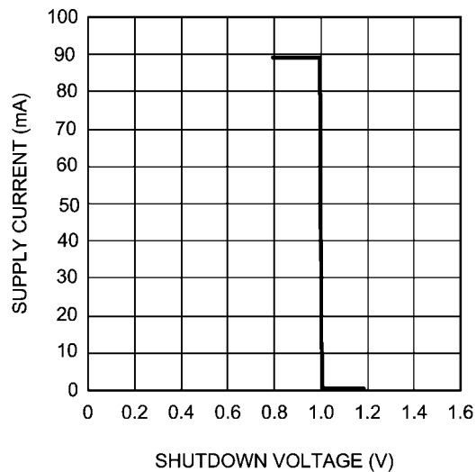
Shutdown Voltage V_{SDIL} V_{DD} = 3.6V
