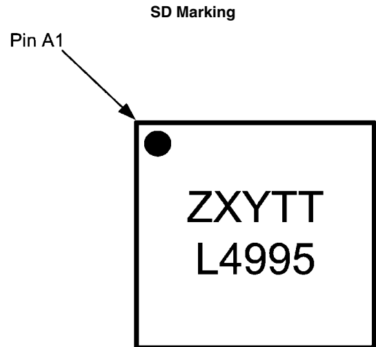
Top View Z - Assembly Plant code XY - 2 Digit date code TT - Die Traceability L4995 - LM4995SD
