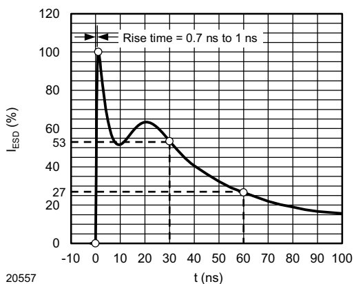
Fig. 1 - 8/20 \mu\text{s} Peak Pulse Current Wave Form (acc. IEC 61000-4-5)
