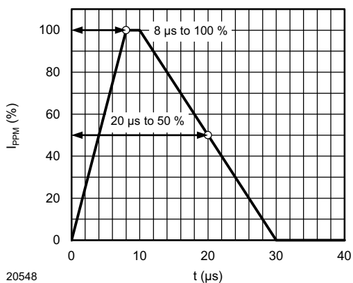
Fig. 2 - ESD Discharge Current Wave Form acc. IEC 61000-4-2 (330 \Omega /150 pF)
