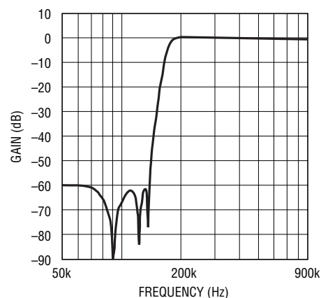
Amplitude Response
