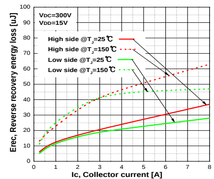
Typ. Reverse recovery energy loss
