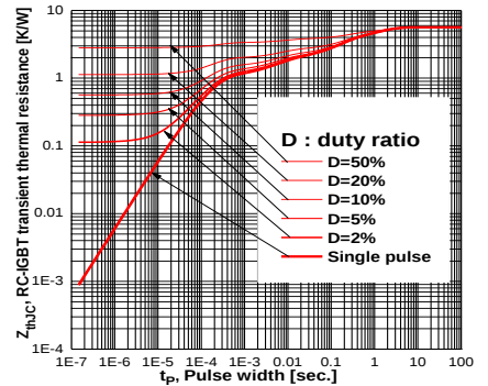
Typ. IGBT transient thermal resistance at all six IGBTs operation
