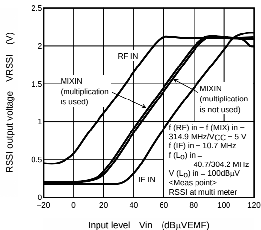
RSSI Output Voltage Characteristics (IF, MIX, and RF inputs)
