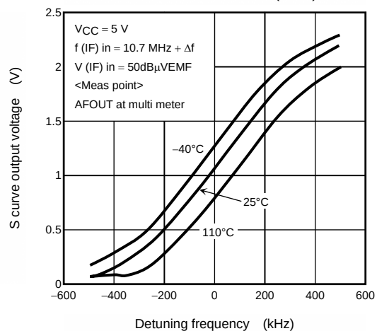
S Curve Characteristics (IF IN)
