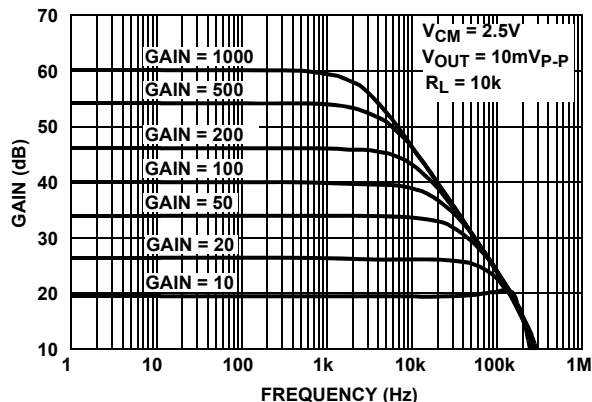
FIGURE 3. ISL28271 FREQUENCY RESPONSE vs CLOSED LOOP GAIN, V_+ = 5V , V_{CM} = 1/2V_+
