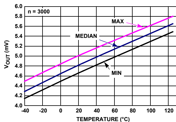
FIGURE 36. ISL28272 V_{OUT} LOW vs TEMPERATURE, R_L = 100k , V_+, V_- = \pm 2.5V
