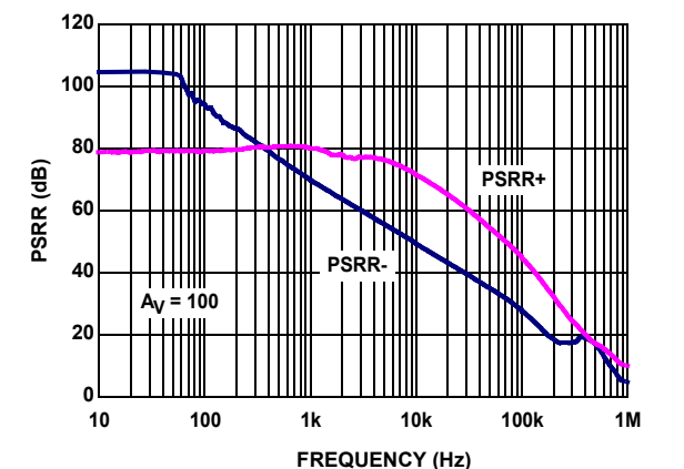
FIGURE 14. ISL28272 PSRR vs FREQUENCY
