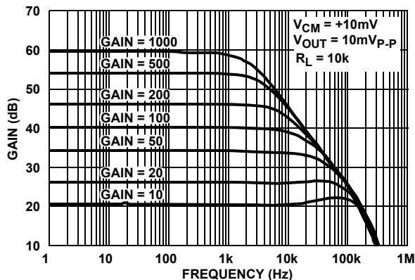
FIGURE 5. ISL28271 FREQUENCY RESPONSE vs CLOSED LOOP GAIN, V_+ = 5V , V_{CM} = 10\text{mV}
