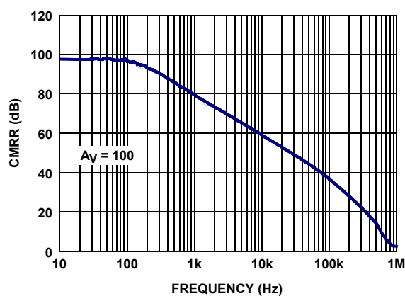
FIGURE 12. ISL28272 CMRR vs FREQUENCY
