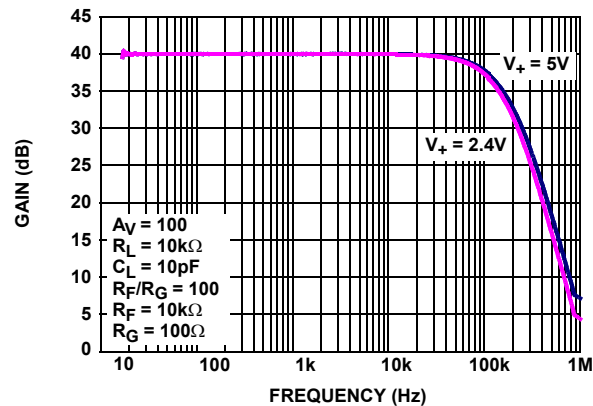
FIGURE 8. ISL28272 FREQUENCY RESPONSE vs SUPPLY VOLTAGE
