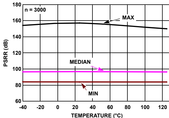
FIGURE 28. ISL28272 PSRR vs TEMPERATURE, V_+ , V_- = \pm 1.2V TO \pm 2.5V
