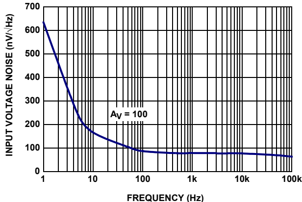
FIGURE 16. ISL28272 INPUT VOLTAGE NOISE SPECTRAL DENSITY
