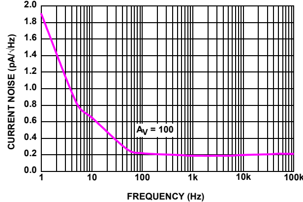
FIGURE 18. ISL28272 INPUT CURRENT NOISE SPECTRAL DENSITY
