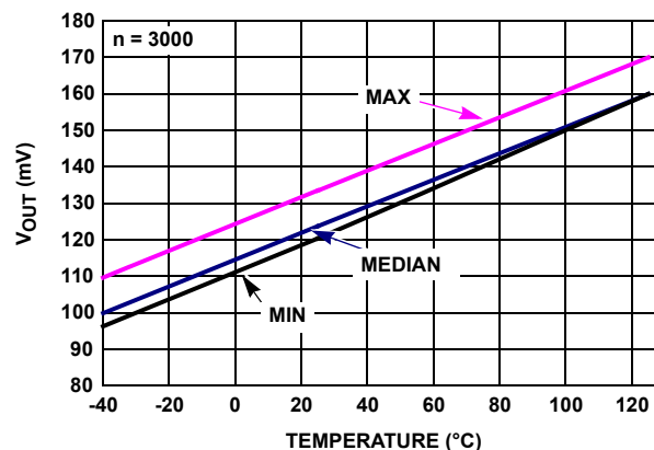
FIGURE 34. ISL28272 V_{OUT} LOW vs TEMPERATURE, R_L = 1k , V_+, V_- = \pm 2.5V
