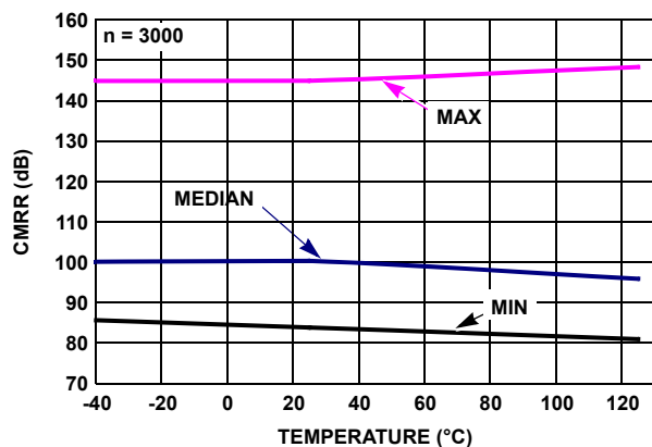
FIGURE 25. ISL28271 CMRR vs TEMPERATURE, V_{CM} = +2.5V TO -2.5V
