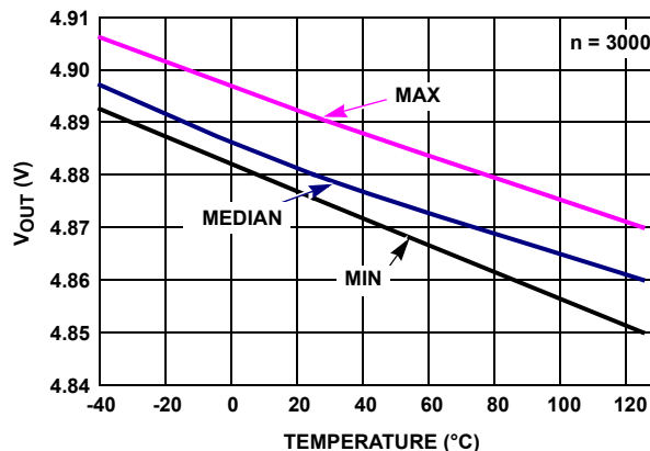
FIGURE 30. ISL28272 V_{OUT} HIGH vs TEMPERATURE, R_L = 1k , V_+ , V_- = \pm 2.5V
