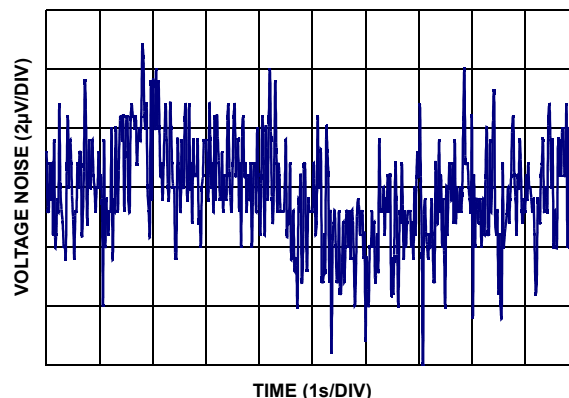
FIGURE 20. ISL28272 0.1Hz TO 10Hz INPUT VOLTAGE NOISE, GAIN = 100
