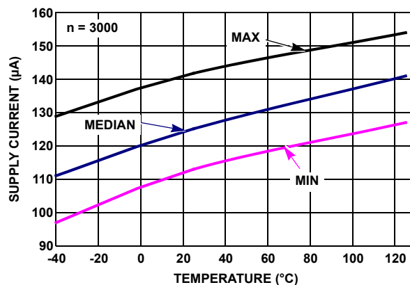
FIGURE 22. ISL28272 SUPPLY CURRENT ENABLED vs TEMPERATURE, V_+ , V_- = \pm 2.5V , V_{IN} = 0V
