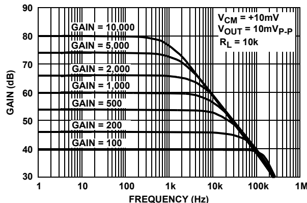
FIGURE 6. ISL28272 FREQUENCY RESPONSE vs CLOSED LOOP GAIN, V_{CM} = V_-
