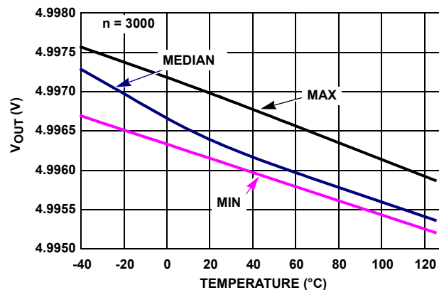
FIGURE 32. ISL28272 V_{OUT} HIGH vs TEMPERATURE, R_L = 100k , V_+, V_- = \pm 2.5V
