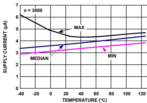
FIGURE 24. ISL28272 SUPPLY CURRENT DISABLED vs TEMPERATURE, V_+ , V_- = \pm 2.5V , V_{IN} = 0V
