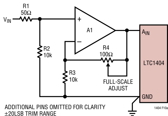
Figure 10a. LTC1404 Full-Scale Adjust Circuit
