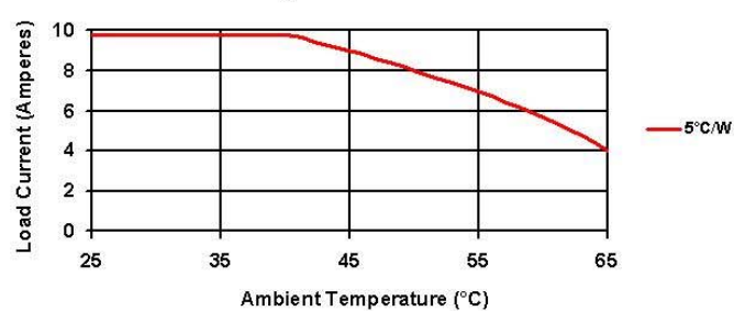
Derating Curve: DC200A10
