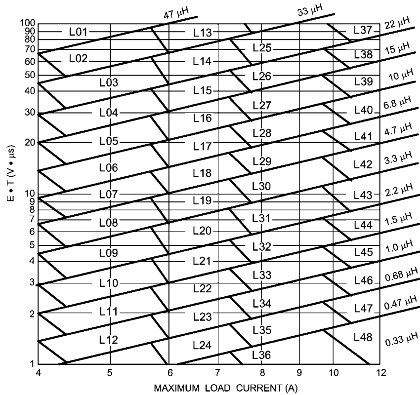
FIGURE 2. Inductor Nomograph
