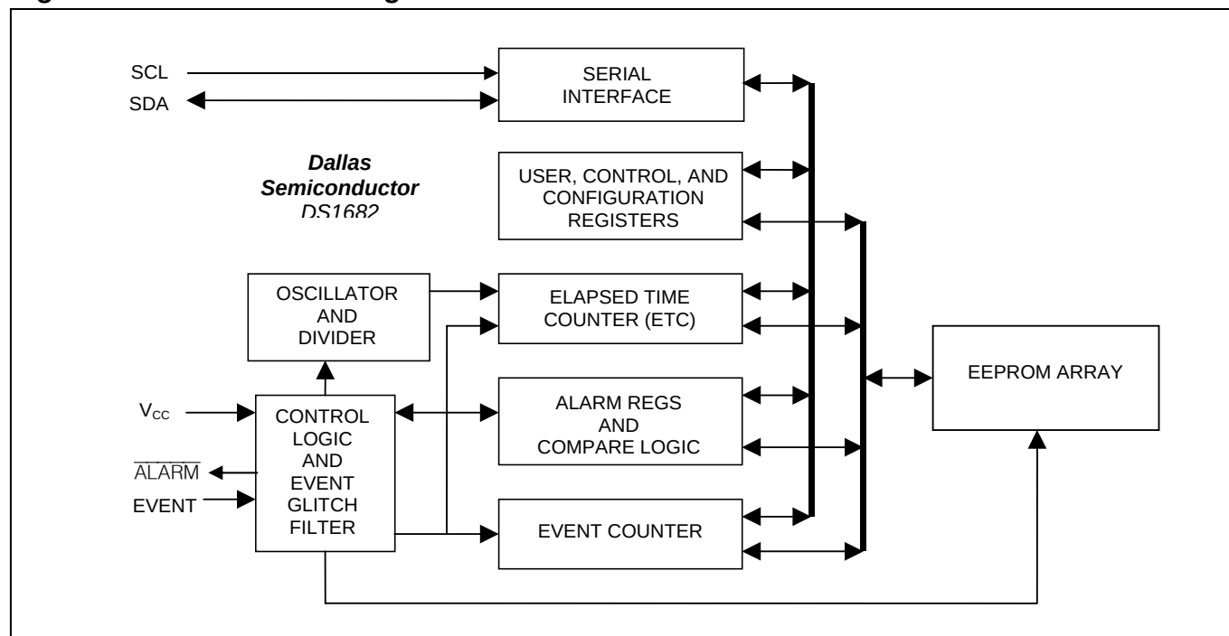
Figure 1. DS1682 Block Diagram
