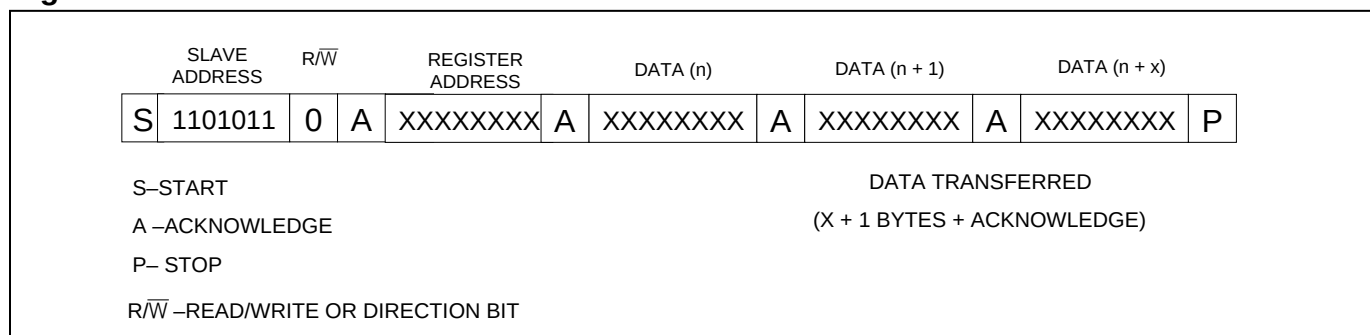
Figure 7. Data Write—Slave Receiver Mode
