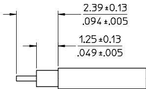
RECOMMENDED STRIP DIMENSIONS
