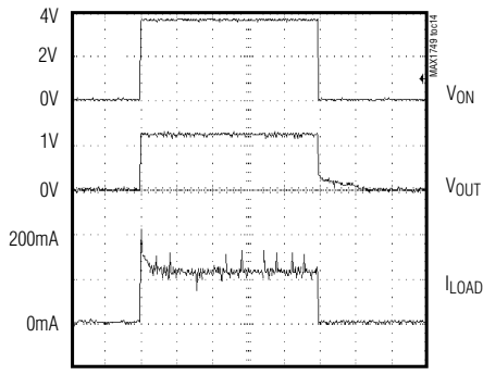
ON/OFF WAVEFORM ( V_{IN} = 3.6V )
