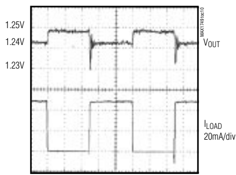
LOAD-TRANSIENT RESPONSE
