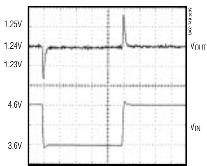
LINE-TRANSIENT RESPONSE
