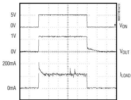
ON/OFF WAVEFORM ( V_{IN} = 5.0V )
