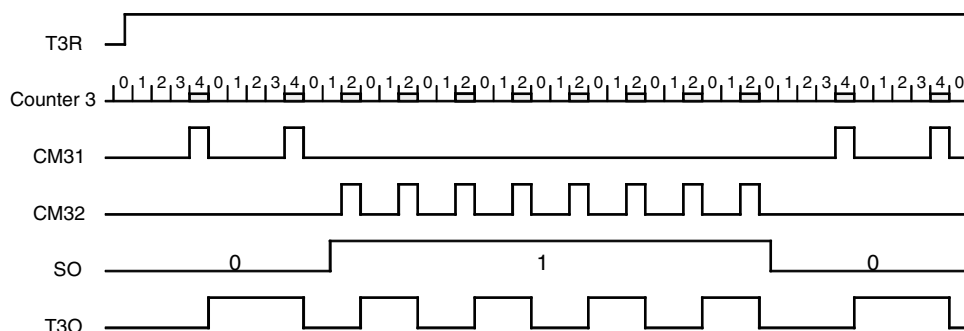
Figure 80. FSK Modulation
