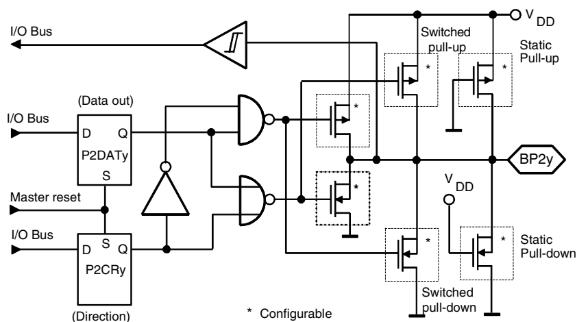
Figure 29. Bi-directional Port 2
