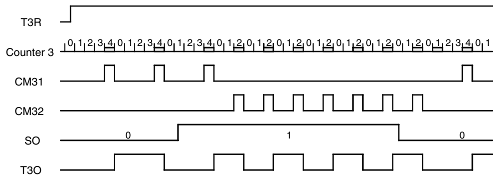
Figure 90. FSK Modulation
