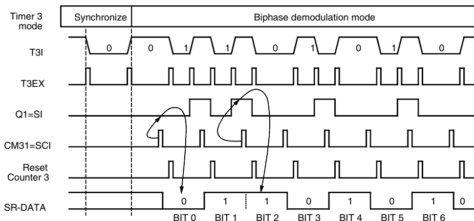
Figure 60. Biphase Demodulation
