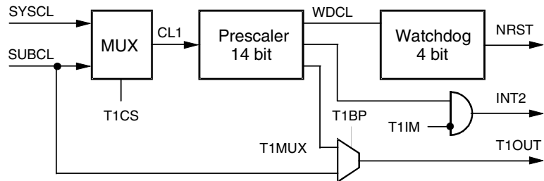
Figure 34. Timer 1 Module
