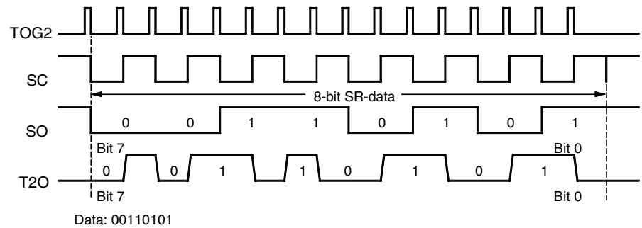
Figure 76. Manchester Modulation 1
