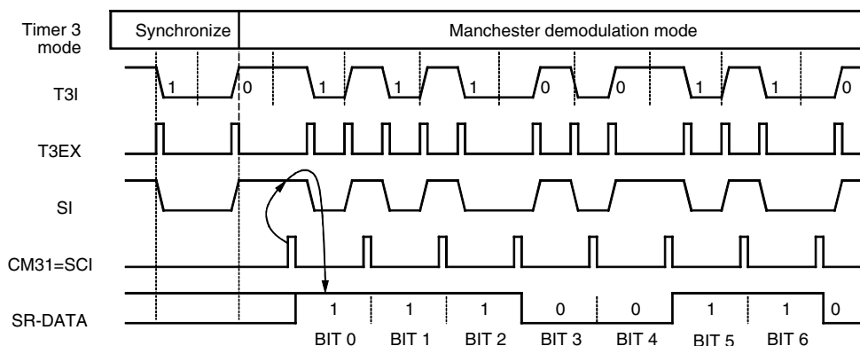
Figure 59. Manchester Demodulation
