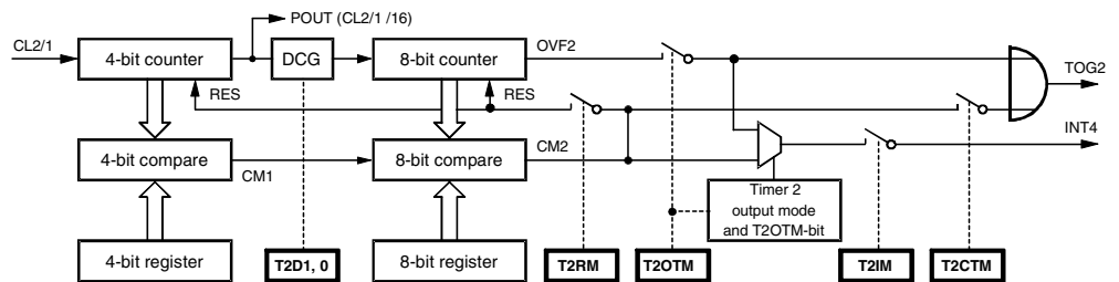
Figure 38. 8-bit Compare Counter
