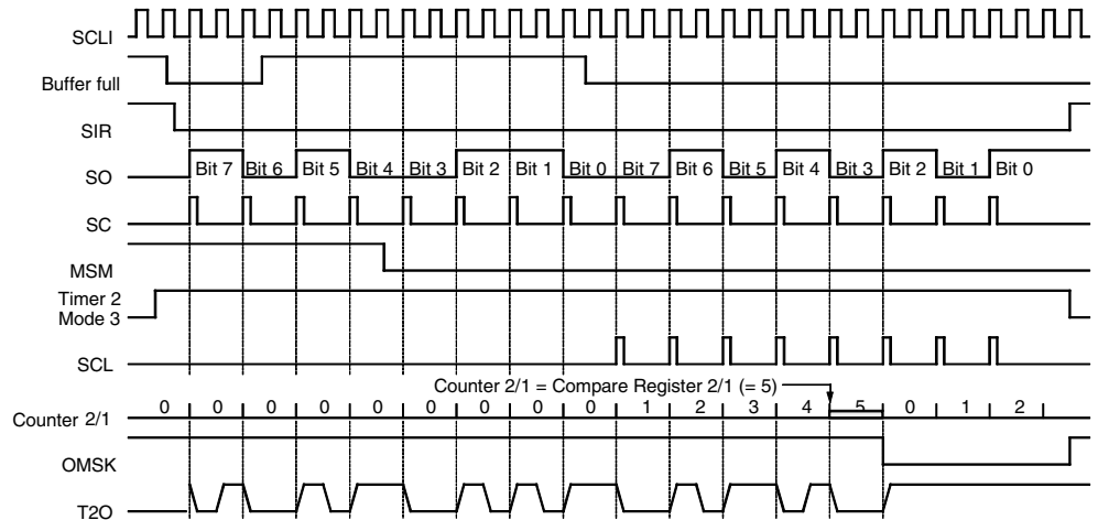
Figure 78. Biphase Modulation 2
