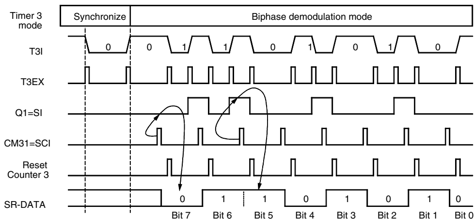
Figure 83. Biphase Demodulation
