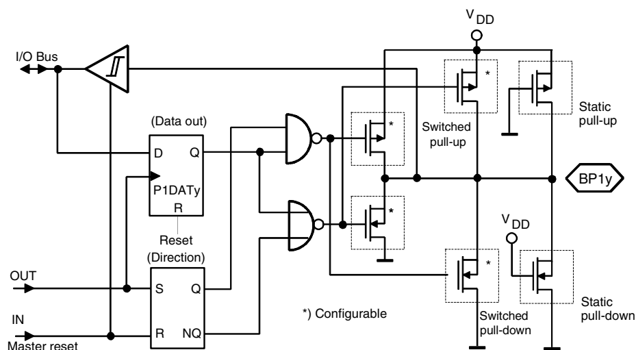
Figure 28. Bi-directional Port 1
