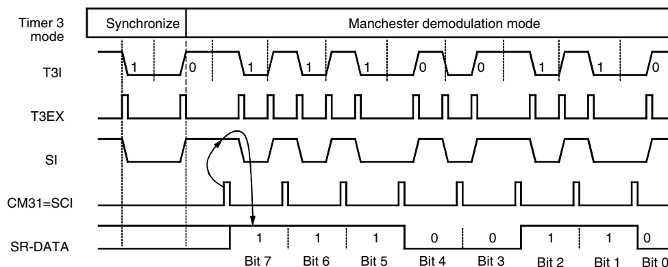
Figure 82. Manchester Demodulation
