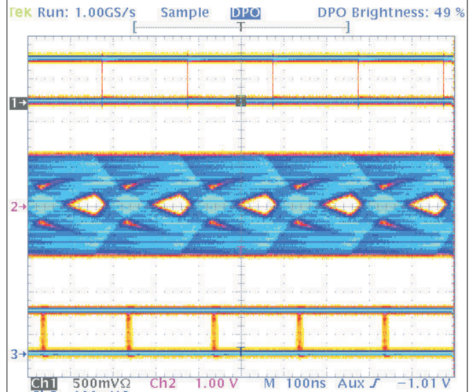
Figure 11-3. SN65HVD24 Receiver Performance at 5 Mbps Over 500 Meter Cable
