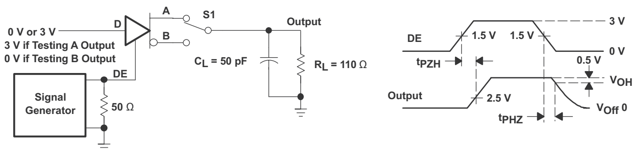
Figure 9-6. Driver Enable and Disable Test, High Output
