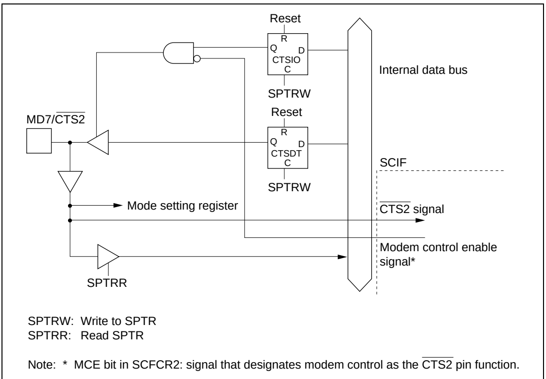
Figure 18.9 MD7/CTS2 Pin
